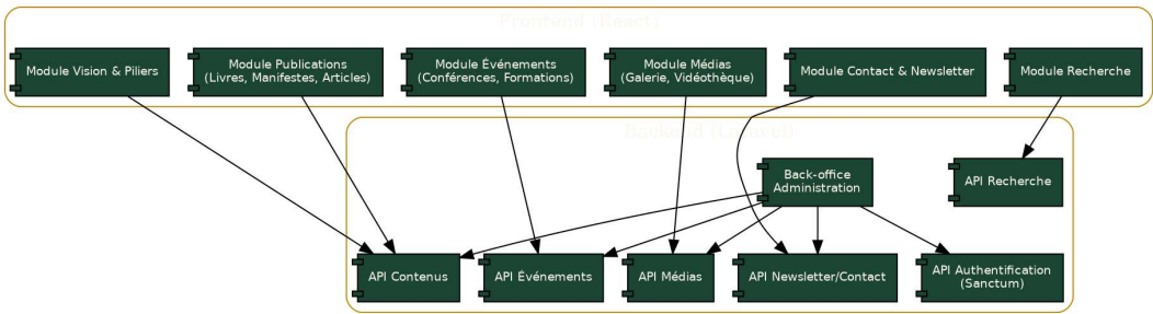
Figure 8 — Diagramme de composants
