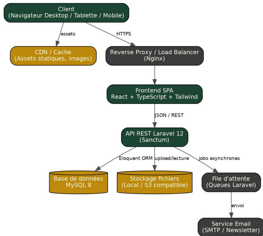
Figure 1 — Architecture applicative globale de la plateforme
